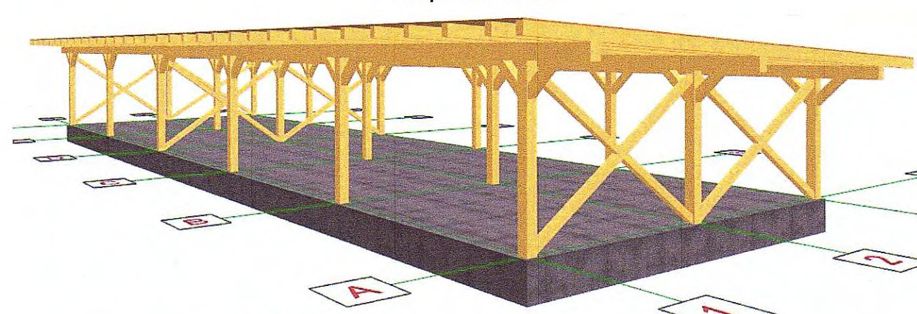
Perspectiva 3D
