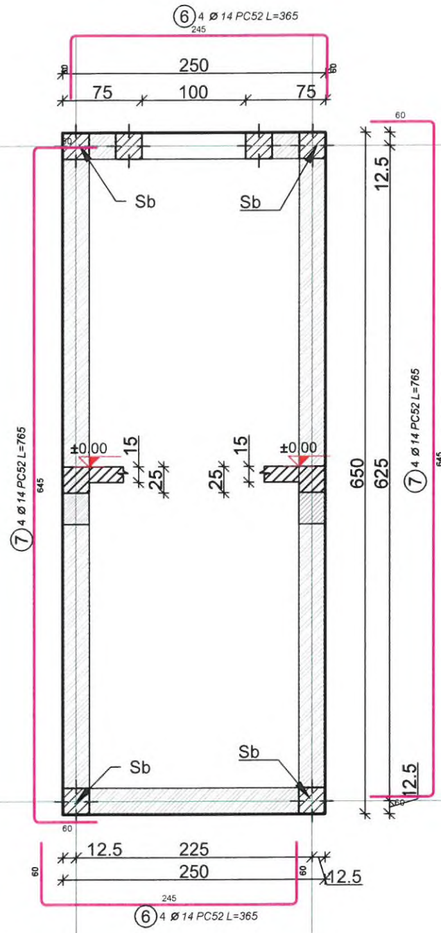
Plan cofraj 1:50 Adapost subteran 2
