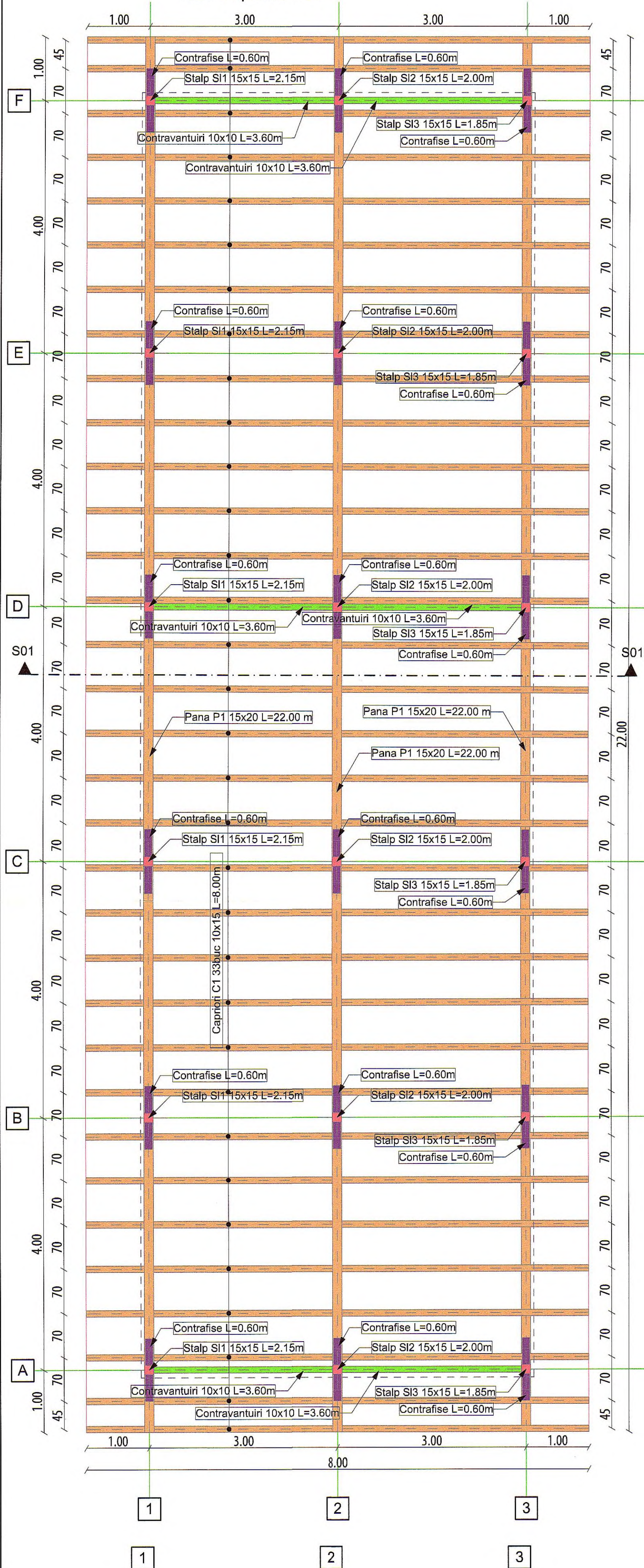
Plan sarpanta 1:50
