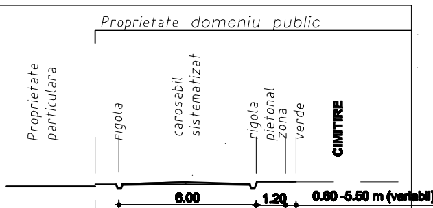
profil transversal caracteristic existent (aprobat prin doc. de urbanism) STRADA CARIEREI
